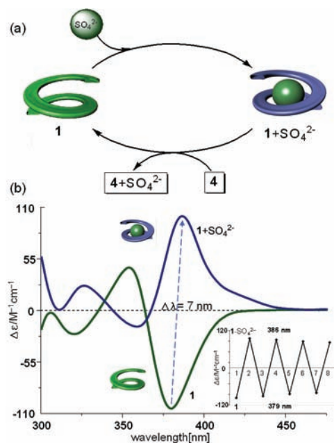
Figure 3. (a) Schematic representation of the reversible switching of the helical sense of 1 upon addition and removal of sulfate ion. (b) CD spectra of unbound 1 (green) and its sulfate complex (blue) and (inset) a repetitive CD cycle upon addition of sulfate or the sulfate-sequestering agent 4 .
